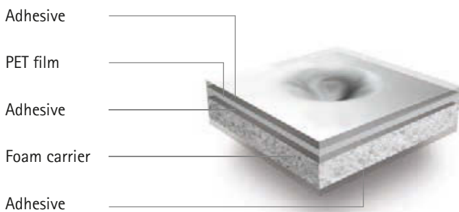
Conventional foam adhesive tape with laminated PET film
