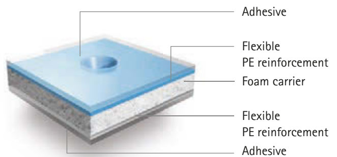
The DuploFLEX® 5 range with double-sided flexible PE reinforcement which perfectly cushions the impression applied and prevents dot gain.
